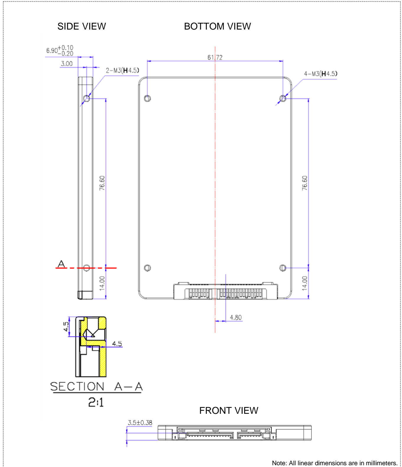
Figure 2-1: 2.5" Industrial SSD Dimensions
