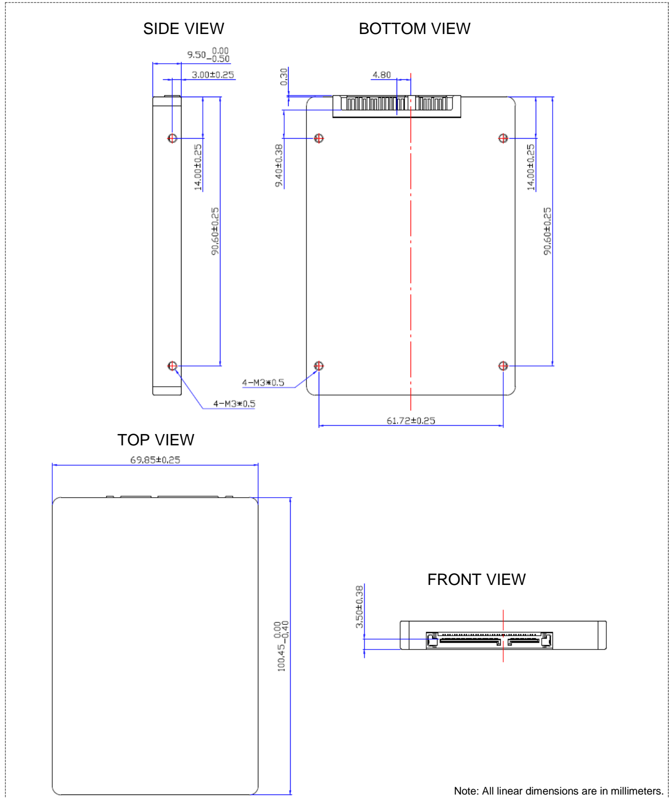
Figure 2-1: U.2 Industrial Enterprise SSD Dimensions
