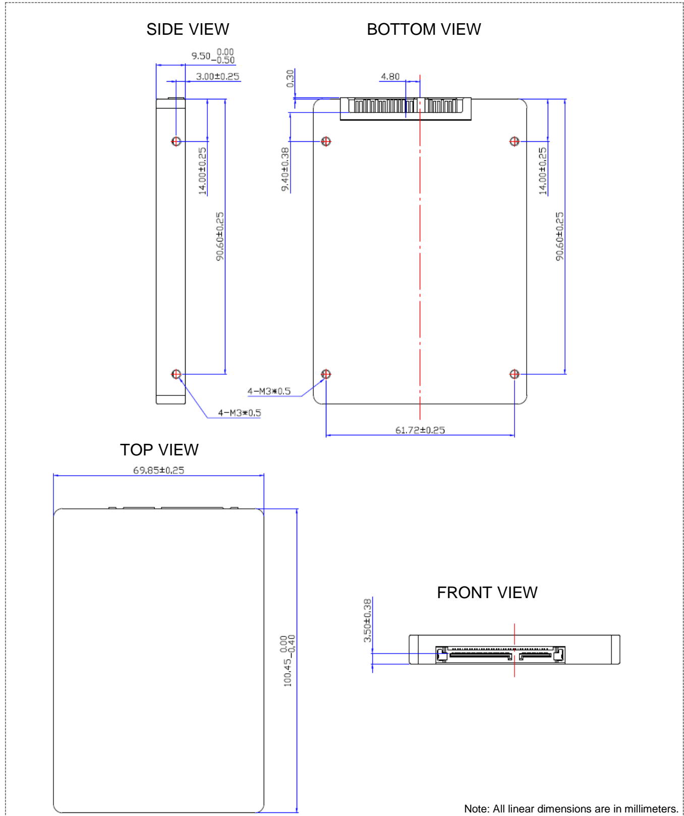
Figure 2-1: 2.5" Industrial Enterprise SSD Dimensions
